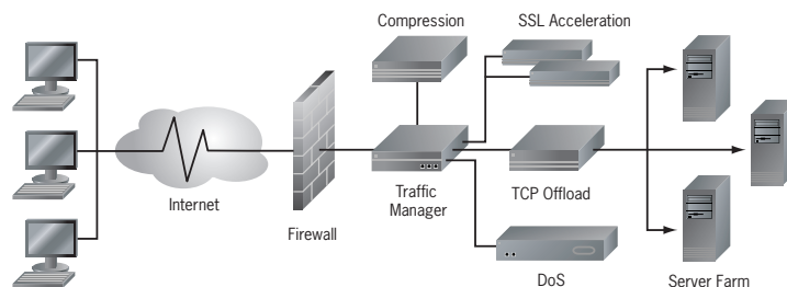
Figure 1: A typical application infrastructure
